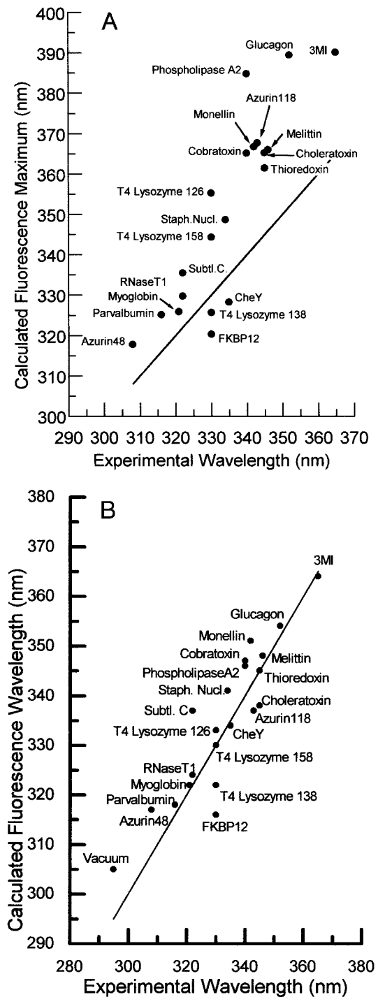
FIGURE 2 Plots of calculated versus experimental fluorescence maximum wavelengths for 19 Trps in 16 proteins and for 3-methylindole in water. (A) Charges on the Trp ring are not scaled and the calculated values are averages over the 400 values during 4 ps of excited-state trajectory. (B) Charges on the Trp ring are multiplied by 0.80 and the calculated values are averages over the 2400 values calculated during the last 24 ps of trajectories of the type shown in Fig. 1.
